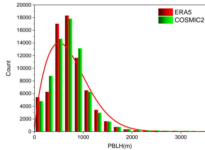
Histogram Plot
