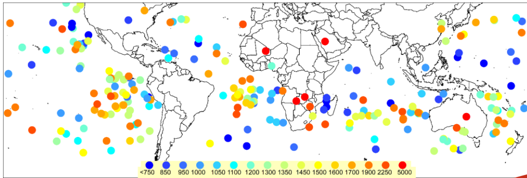
COSMIC2 PBLH
