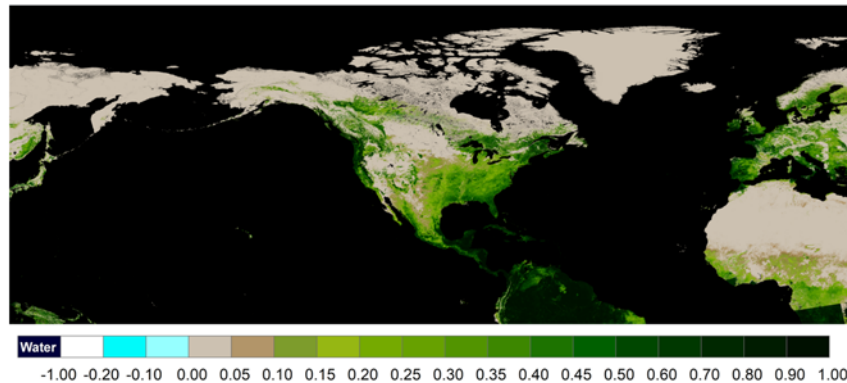
Figure 3-4 Example of regional color-coded 0.009° GVF GeoTIFF produced from a weekly composited VIIRS data 01/03/2018-01/09/2018.
