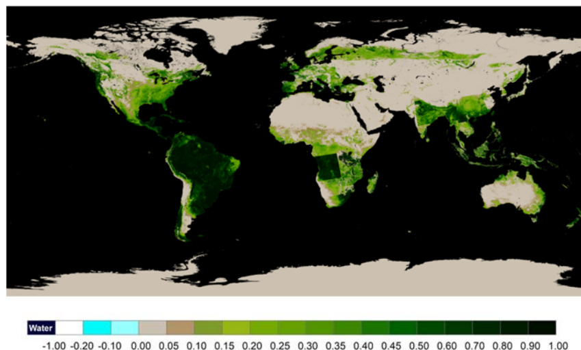
Figure 3-3 Example of global color-coded 0.036° GVF GeoTIFF produced from a weekly composited VIIRS data 01/03/2018-01/09/2018.
