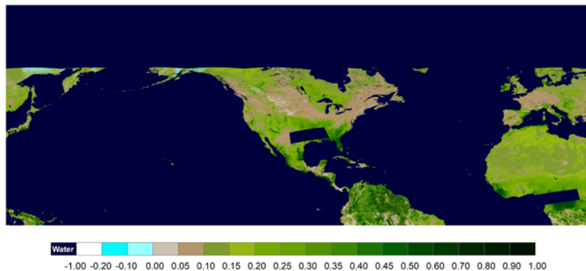
Figure 3-2 (a,b,c) Examples of regional color-coded 0.009° EVI_TOC,NDVI_TOC, NDVI_TOA GeoTIFF produced for 01/04/2018
